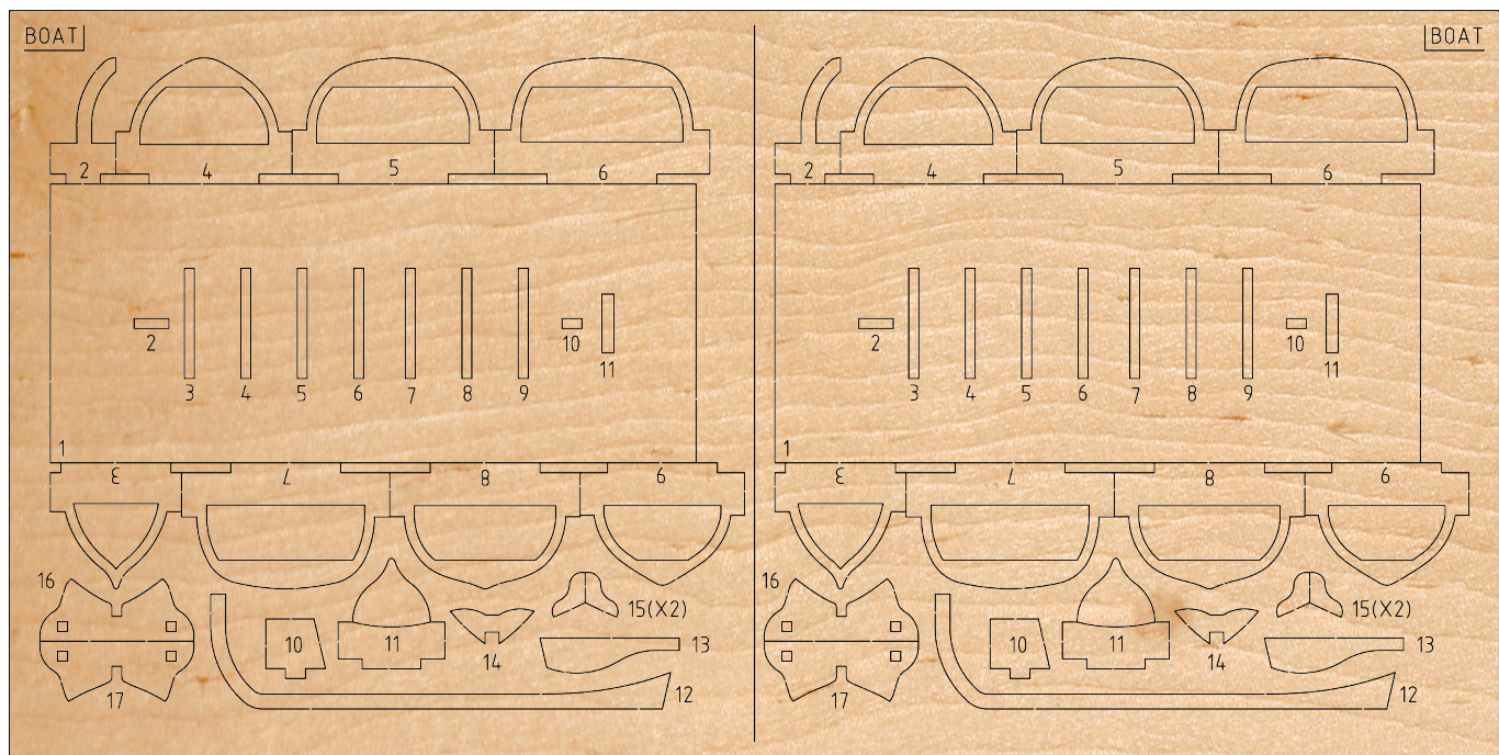
2mm plywood part 300x150mm
