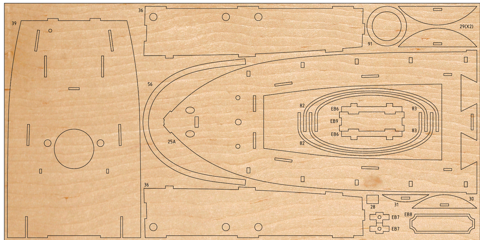
2mm plywood part 450x225mm
